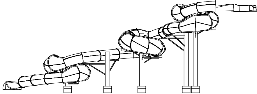
ELEVATION VIEW
