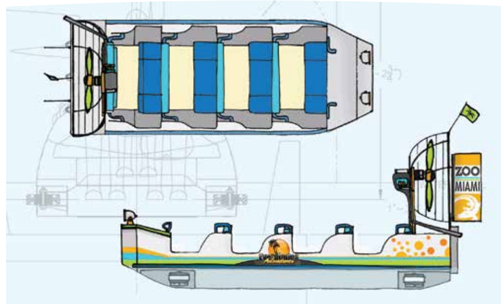
Custom boat design for Zoo Miami, Miami, Florida
