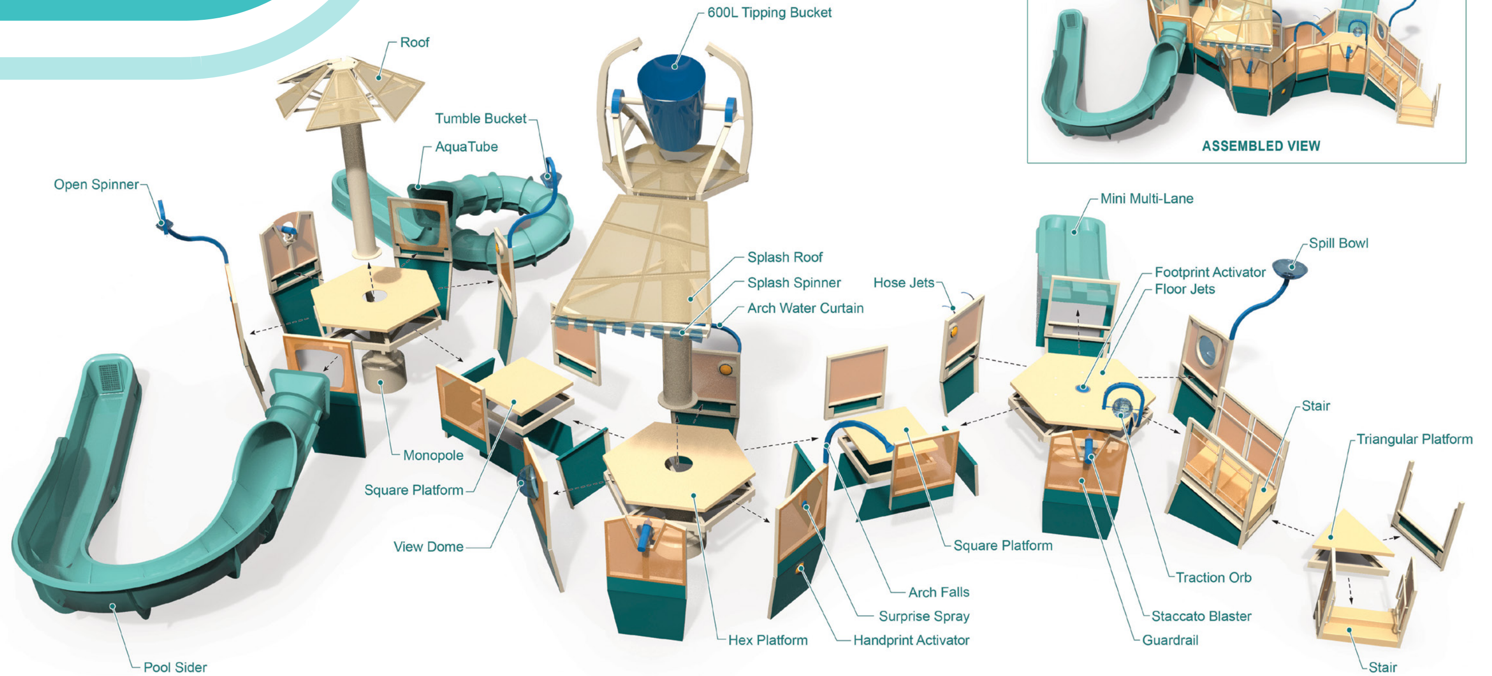
EXPLODED VIEW
